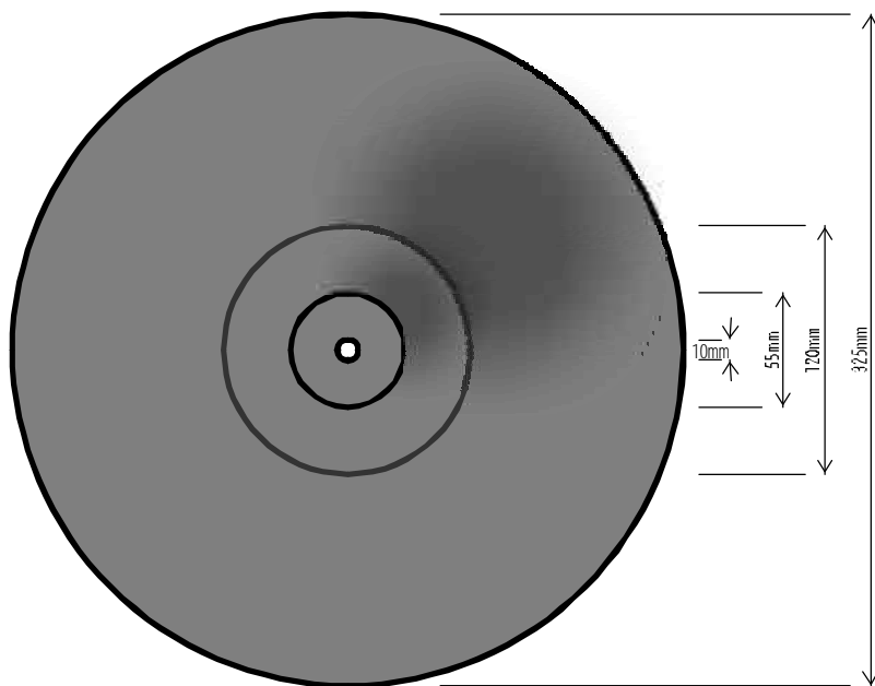
MEDIUM BASE
