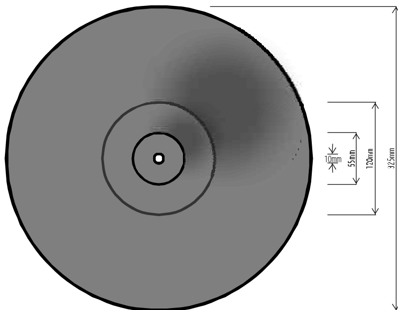
MEDIUM BASE
