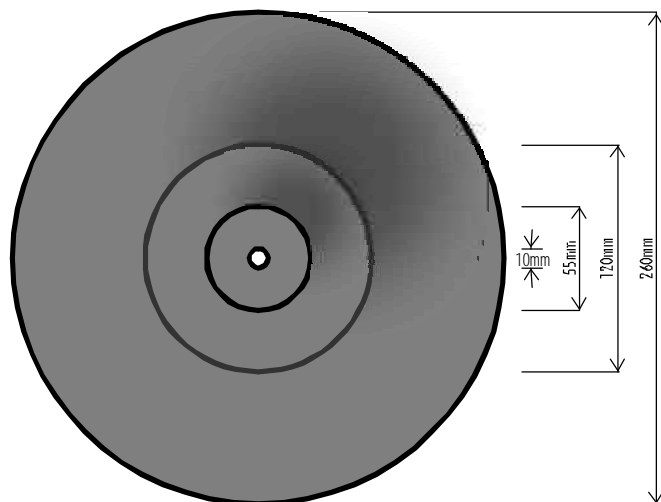
SMALL BASE
